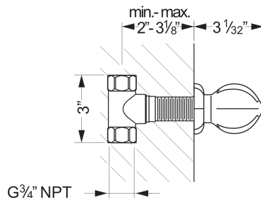
shown with R1040R 3/4" volume control
