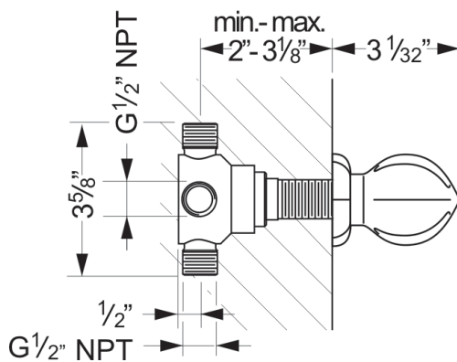
shown with R1062BO 4-port diverter
