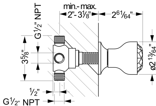
shown with R1062BO 4-port diverter
