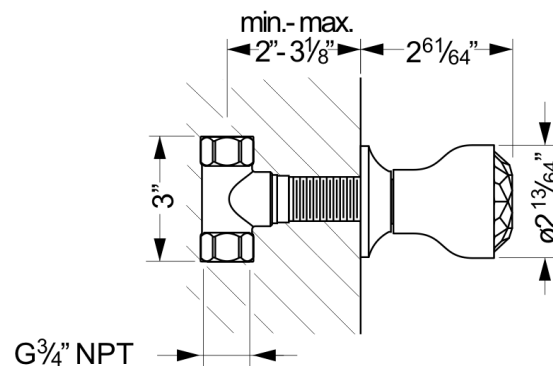
shown with R1040R 3/4" volume control
