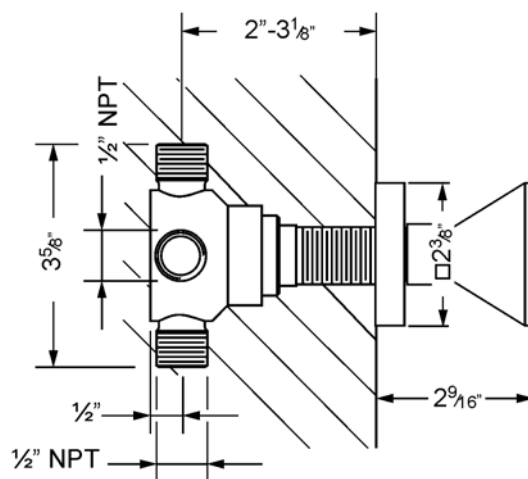
with concealed wall valve 649.40.620.000
